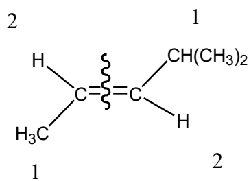
(E)-4-methyl-2-pentene
